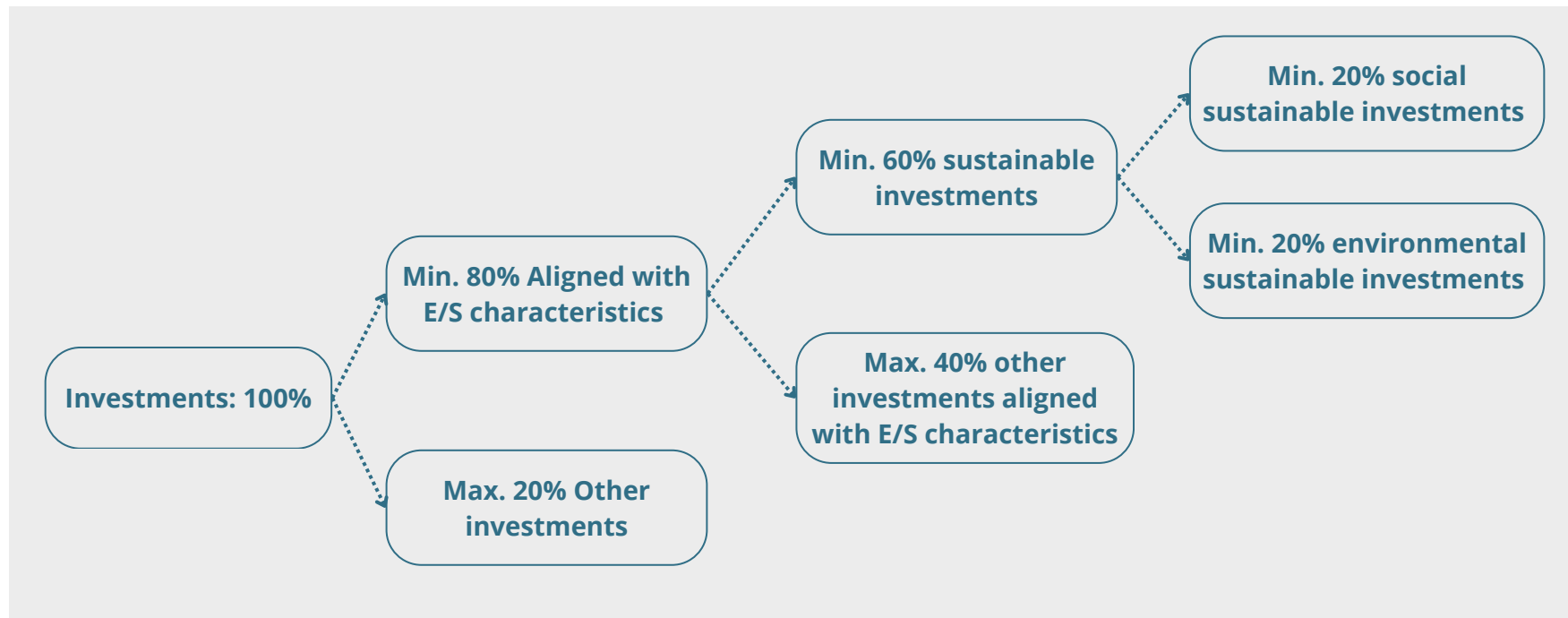
Figure 1: Asset allocation of Smart Convictions
